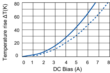
[ ETQP5M150YFK ]
