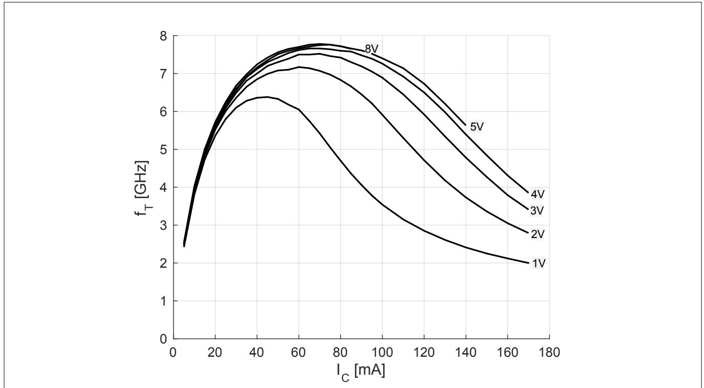
Figure 9 Transition frequency f_T = f(I_C) , V_{CE} = parameter
