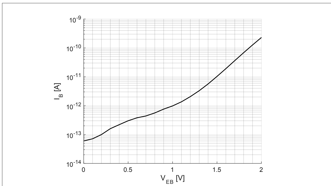
Figure 8 Base/emitter leakage current I_B = f(V_{EB}) , V_{CE} = 8 \text{ V}
