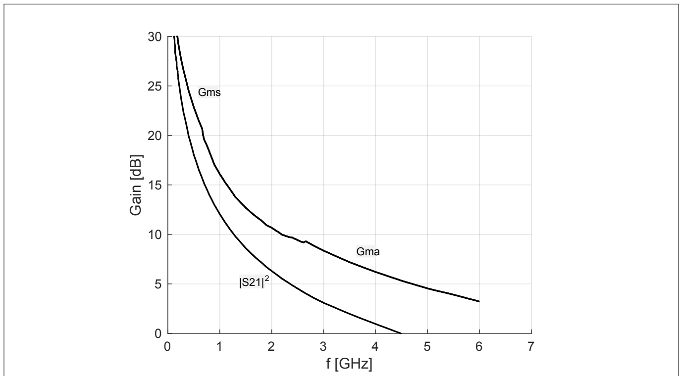
Figure 10 Gain G_{ms} , G_{ma} , |S_{21}|^2 = f(f) , I_C = 50 mA, V_{CE} = 8 V
