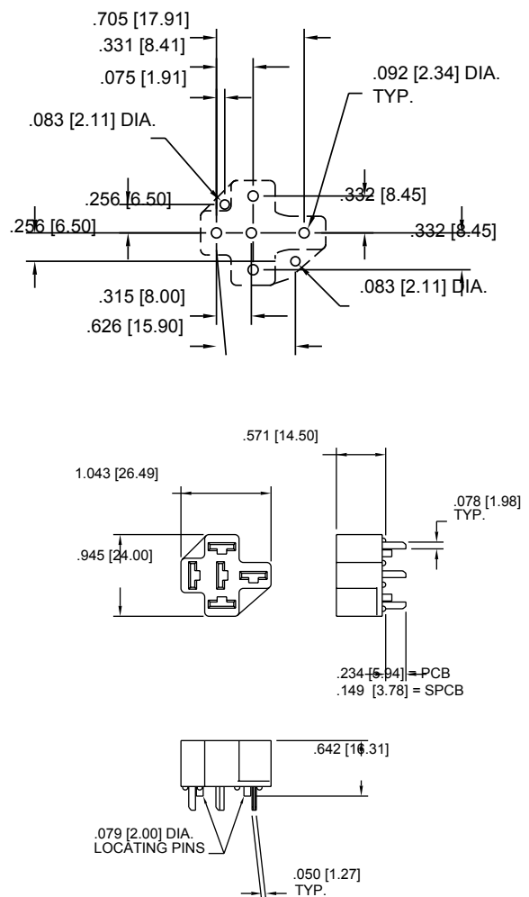
PC BOARD LAYOUT
