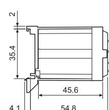
062.07 with relay
