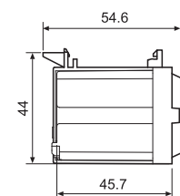
062.08 with relay
