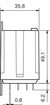
Type 62.8x
