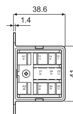
062.60 with relay
