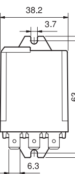
Type 62.83 62.83-0300
