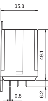
Type 62.8x-0300
