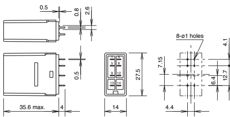
RY2V
