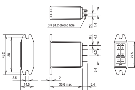
RY2S-UT
