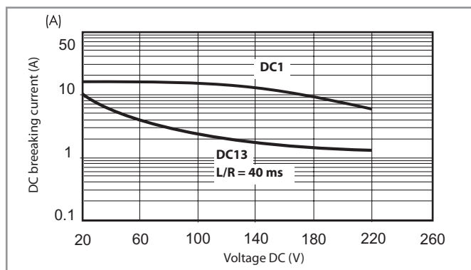
H 62 - Maximum DC breaking capacity 62.32.9.xxx.4800
