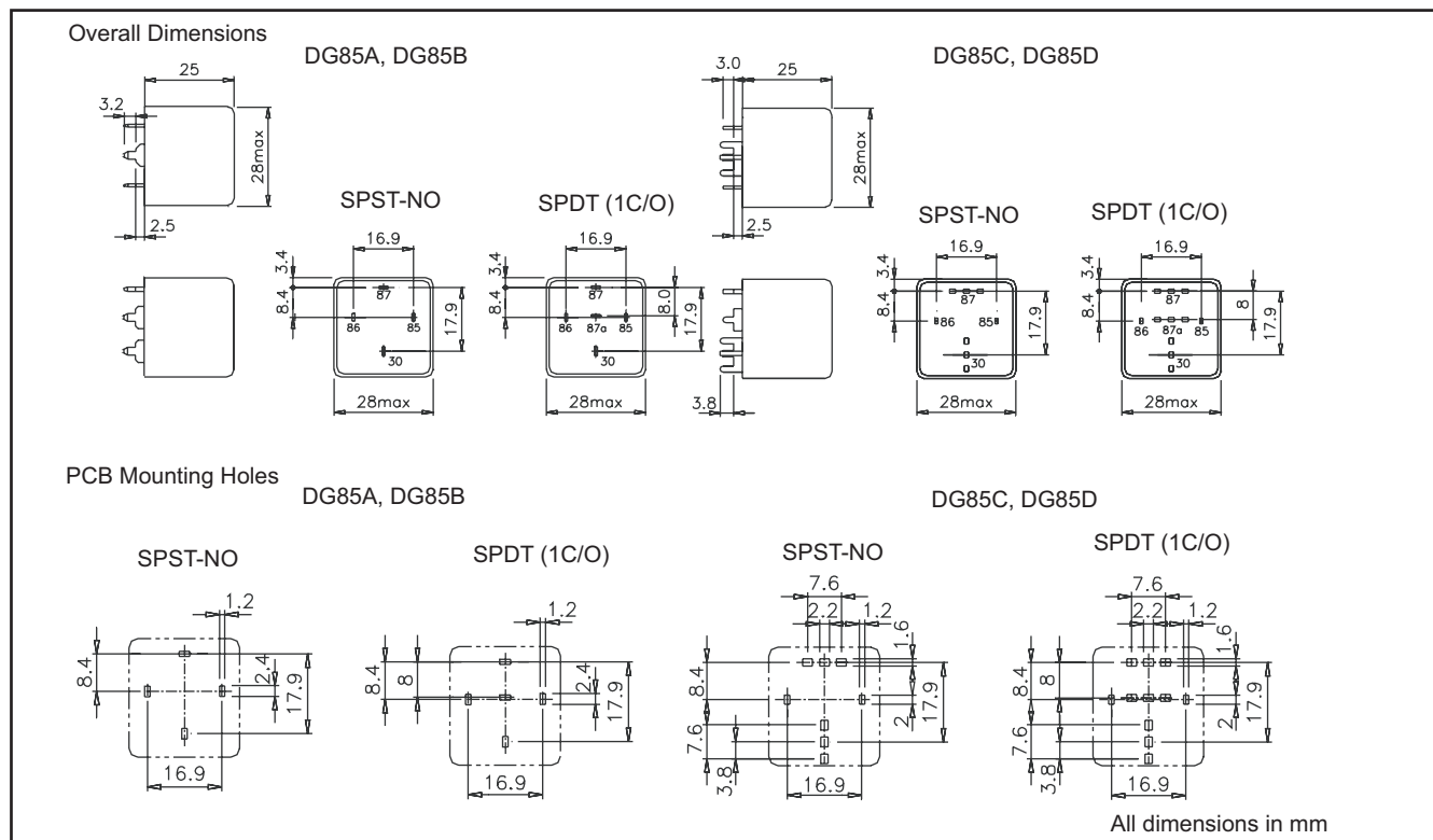
Dimensions - PCB types
