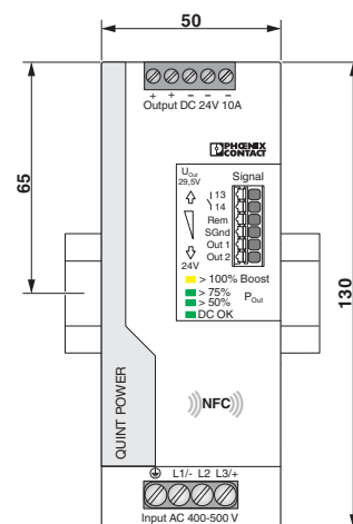
Dimensional drawing
