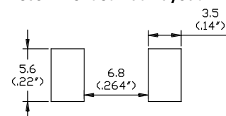
REFLOW SOLDER
