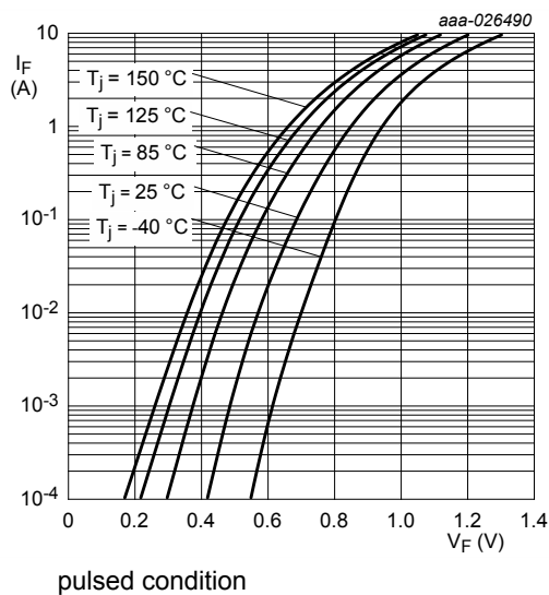
Fig. 3. Forward current as a function of forward voltage; typical values
