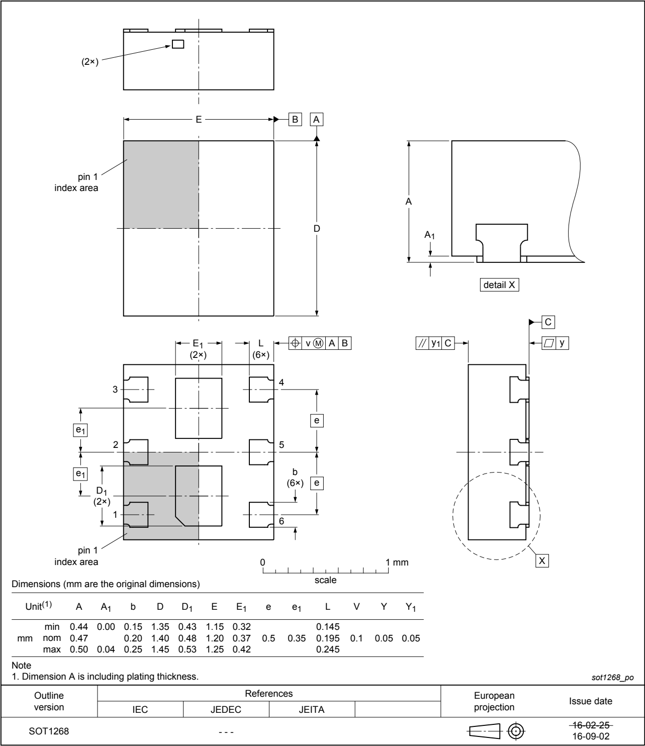
Fig. 9. Package outline DFN1412-6 (SOT1268)
