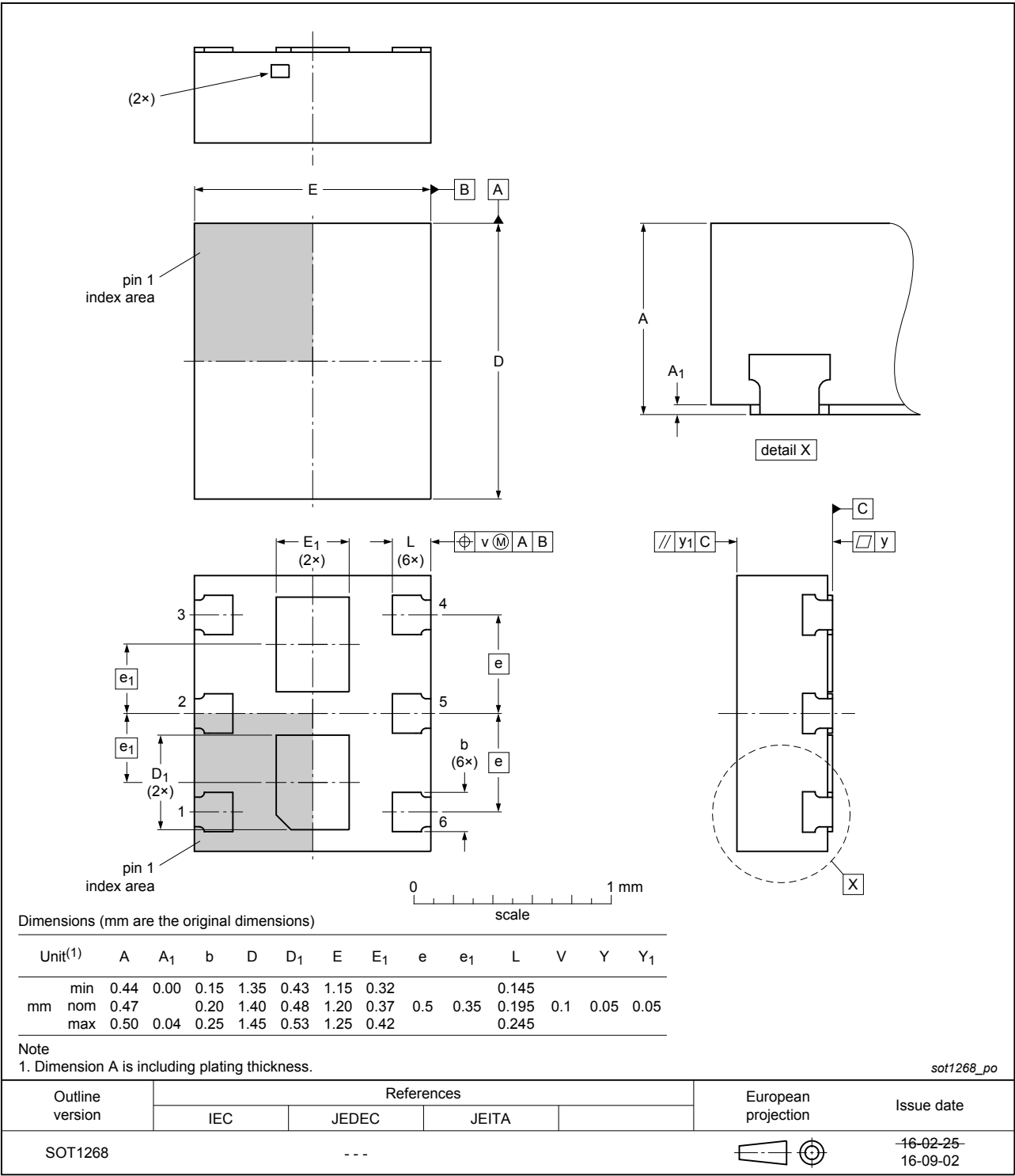
Fig. 8. Package outline DFN1412-6 (SOT1268)
