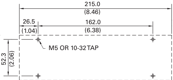
MOUNTING DETAIL
