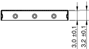
sectional drawing A-A
