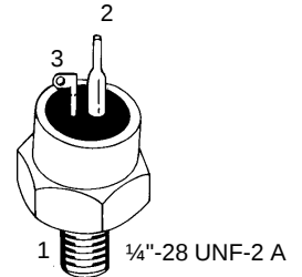
TO-208AC (TO-65)
