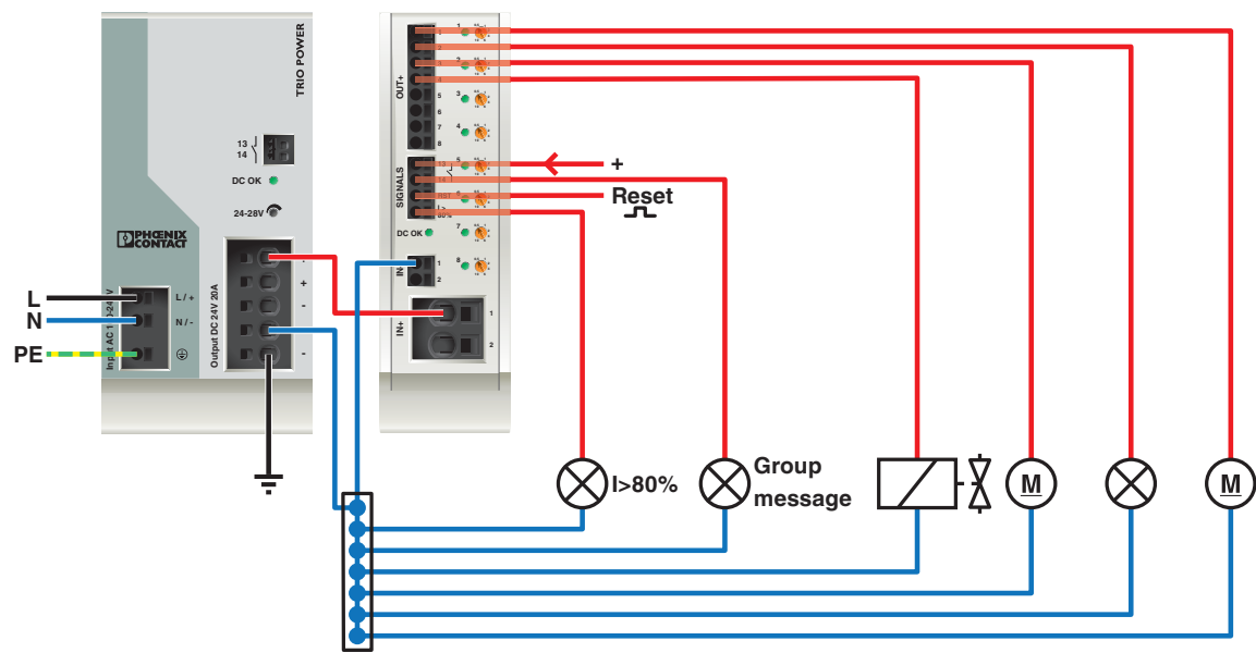
Application drawing
