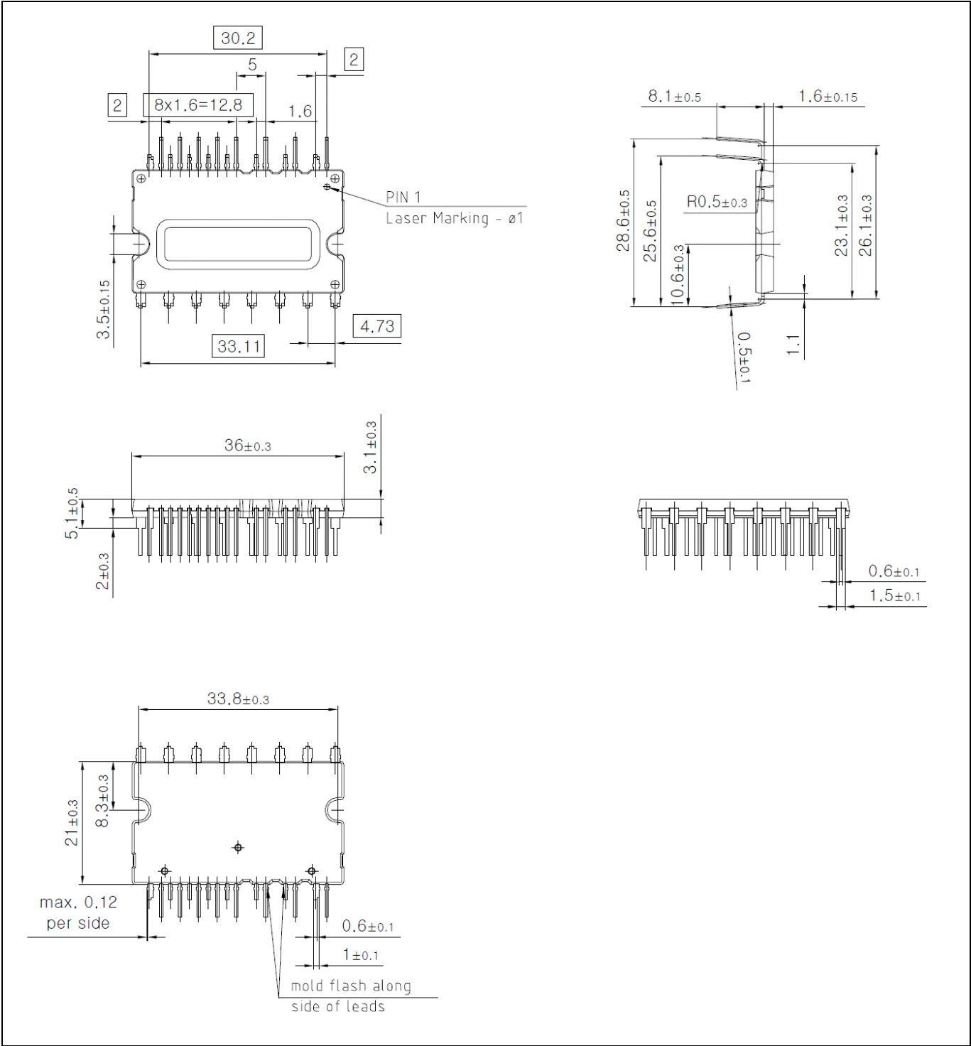
Figure 12 IGCM04F60GA
