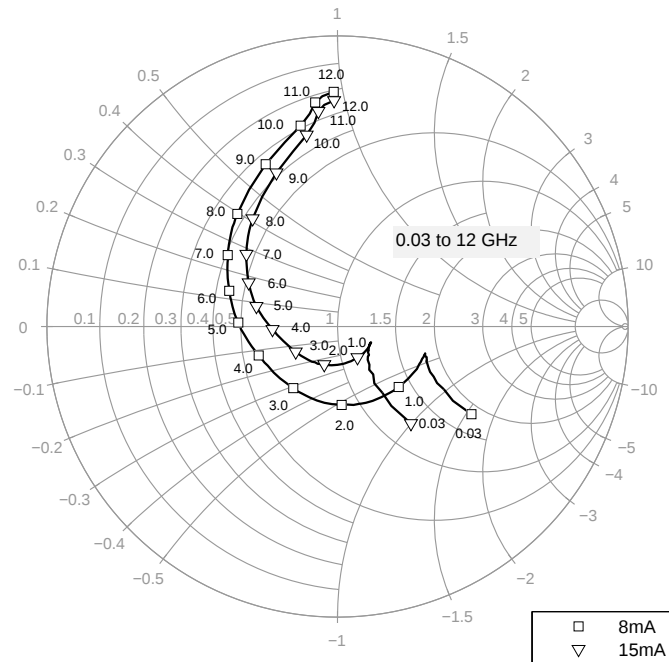
Figure 7-9 Output Reflection Coefficient S_{22} = f(f) , V_{CE} = 1.8 \text{ V} , I_C = 8 / 15 \text{ mA}
