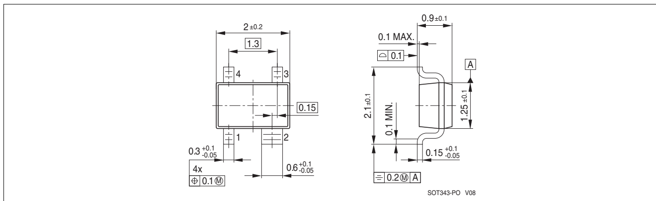
Figure 9-1 Package Outline
