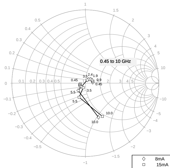
Figure 7-8 Source Impedance for Minimum Noise Figure Z_{opt} = f(f) , V_{CE} = 1.8\text{ V} , I_C = 8 / 15\text{ mA}
