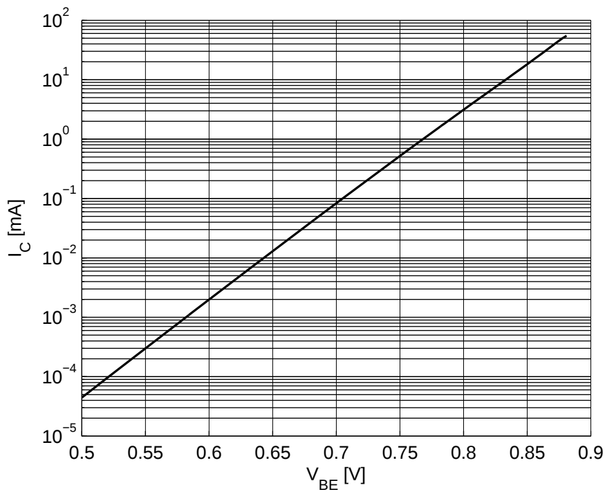
Figure 6-3 Collector Current vs. Base Emitter Forward Voltage I_C = f(V_{BE}) , V_{CE} = 1.8 V
