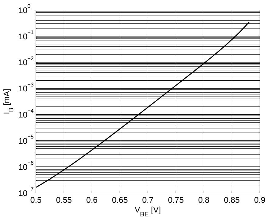
Figure 6-4 Base Current vs. Base Emitter Forward Voltage I_B = f(V_{BE}) , V_{CE} = 1.8 V
