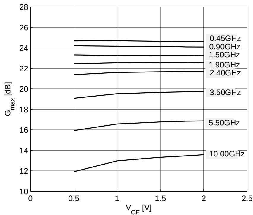
Figure 7-6 Maximum Power Gain G_{max} = f(V_{CE}) , I_C = 15\text{ mA} , f = \text{Parameter in GHz}
