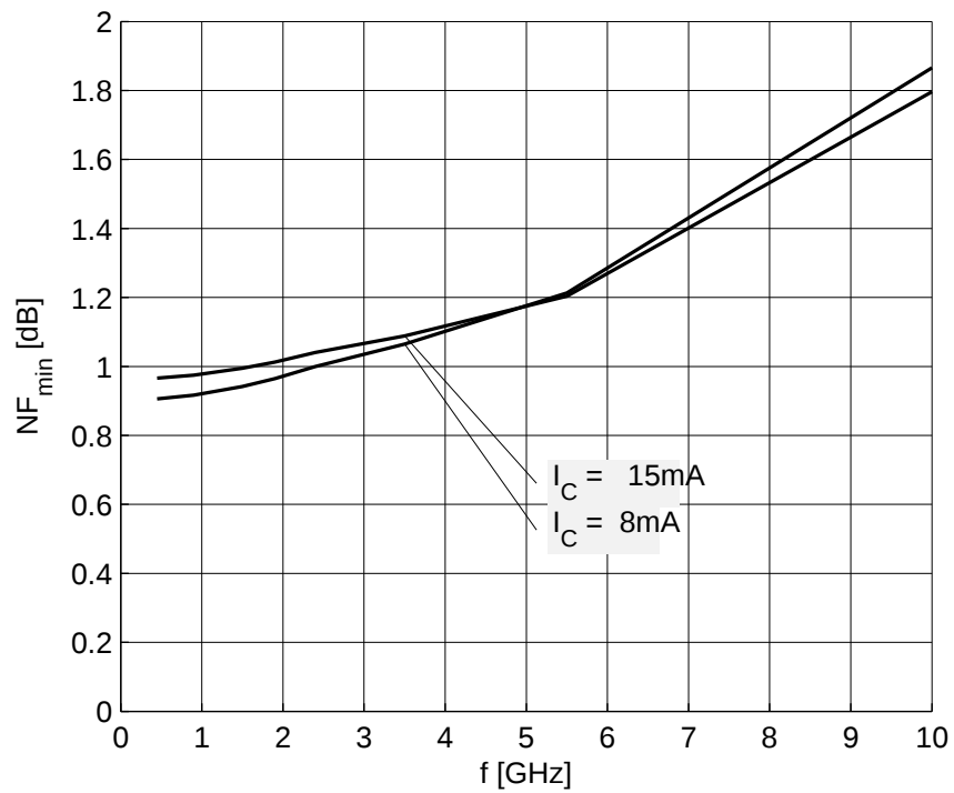
Figure 7-10 Noise Figure NF_{min} = f(f) , V_{CE} = 1.8 \text{ V} , I_C = 8 / 15 \text{ mA} , Z_S = Z_{opt}
