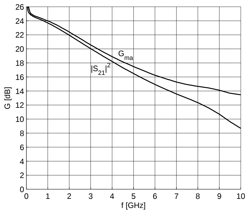
Figure 7-4 Gain G_{ma} , G_{ms} , |S_{21}|^2 = f(f) , V_{CE} = 1.8 \text{ V} , I_C = 15 \text{ mA}
