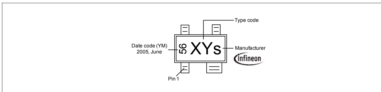
Figure 9-3 Marking Description (Marking BFP843: T2s)
