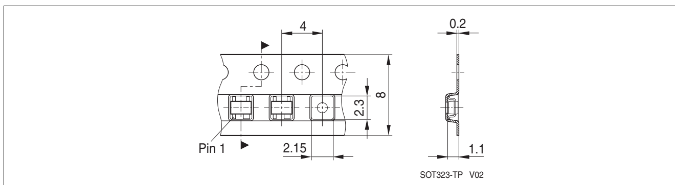
Figure 9-4 Tape Dimensions
