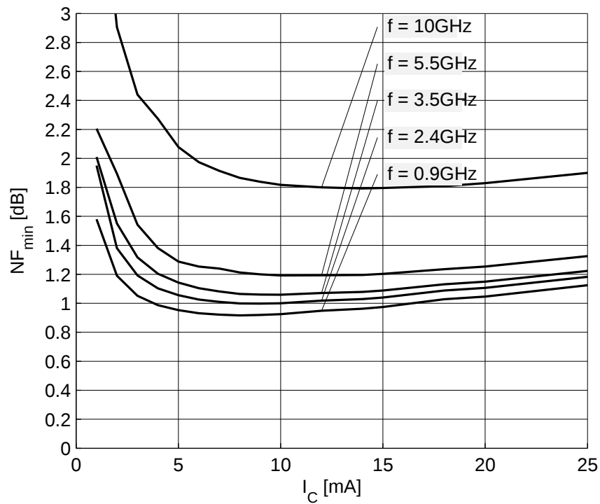
Figure 7-11 Noise Figure NF_{min} = f(I_C) , V_{CE} = 1.8 V, Z_S = Z_{opt} , f = Parameter in GHz
