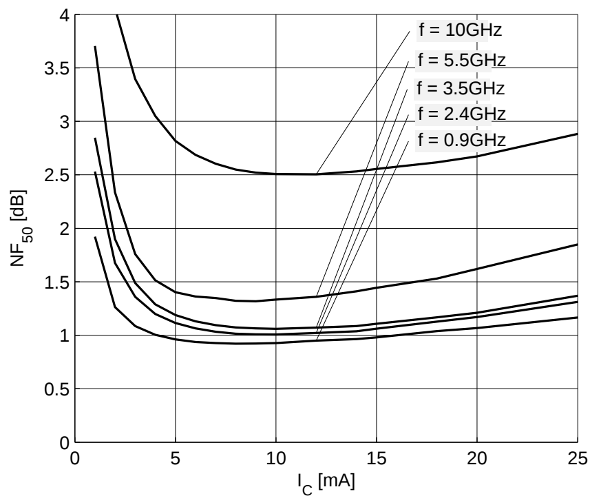
Figure 7-12 Noise Figure NF_{50} = f(I_C) , V_{CE} = 1.8 V, Z_S = 50 \Omega , f = Parameter in GHz
