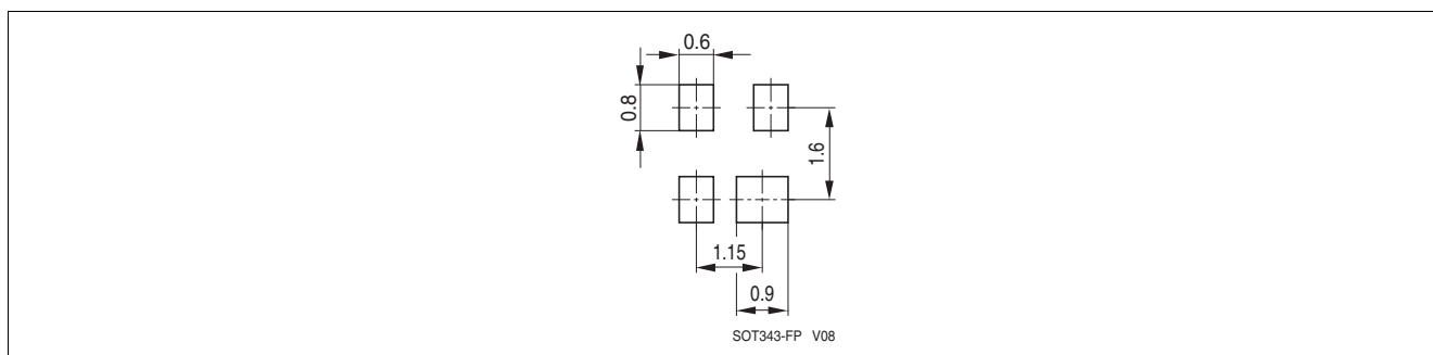
Figure 9-2 Package Footprint
