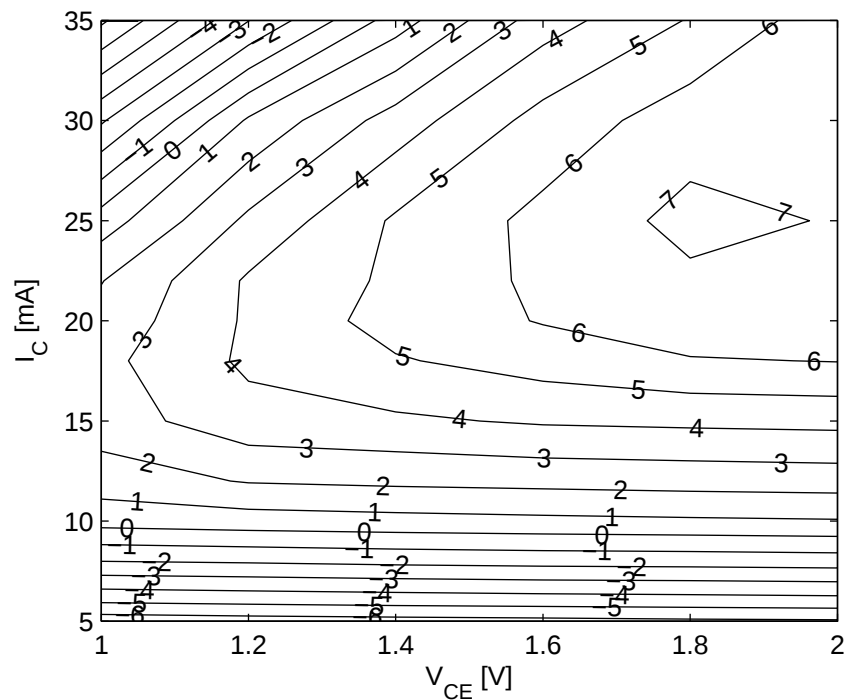
Figure 7-3 Compression Point at Output OP_{1dB} [dBm] = f(I_C, V_{CE}) , Z_S = Z_L = 50 \Omega , f = 5.5 \text{ GHz}
