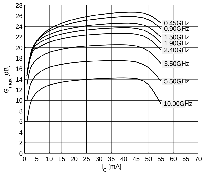
Figure 7-5 Maximum Power Gain G_{max} = f(I_C) , V_{CE} = 1.8\text{ V} , f = \text{Parameter in GHz}
