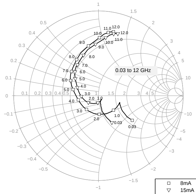
Figure 7-7 Input Reflection Coefficient S_{11} = f(f) , V_{CE} = 1.8\text{ V} , I_C = 8 / 15\text{ mA}
