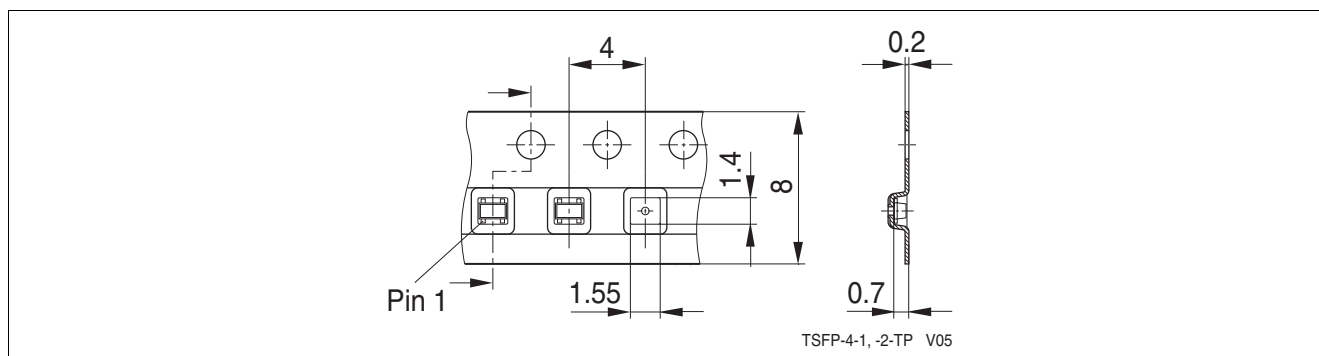
Figure 9-4 Tape dimensions
