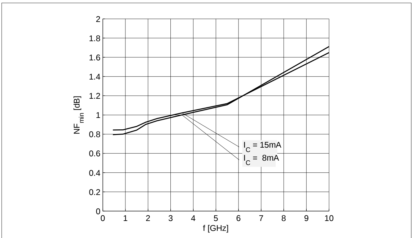
Figure 7-10 Noise Figure NF_{\min} = f(f) , V_{CE} = 1.8 \text{ V} , I_C = 8 / 15 \text{ mA} , Z_S = Z_{\text{opt}}
