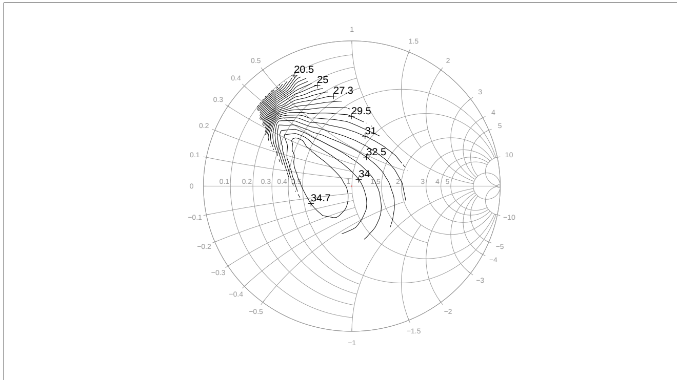
Figure 7-17 Load Pull Contour OIP3 [dBm] at V_{CE} = 5 V, I_C = 90 mA, f = 0.9 GHz, Z_I = Z_{opt}
