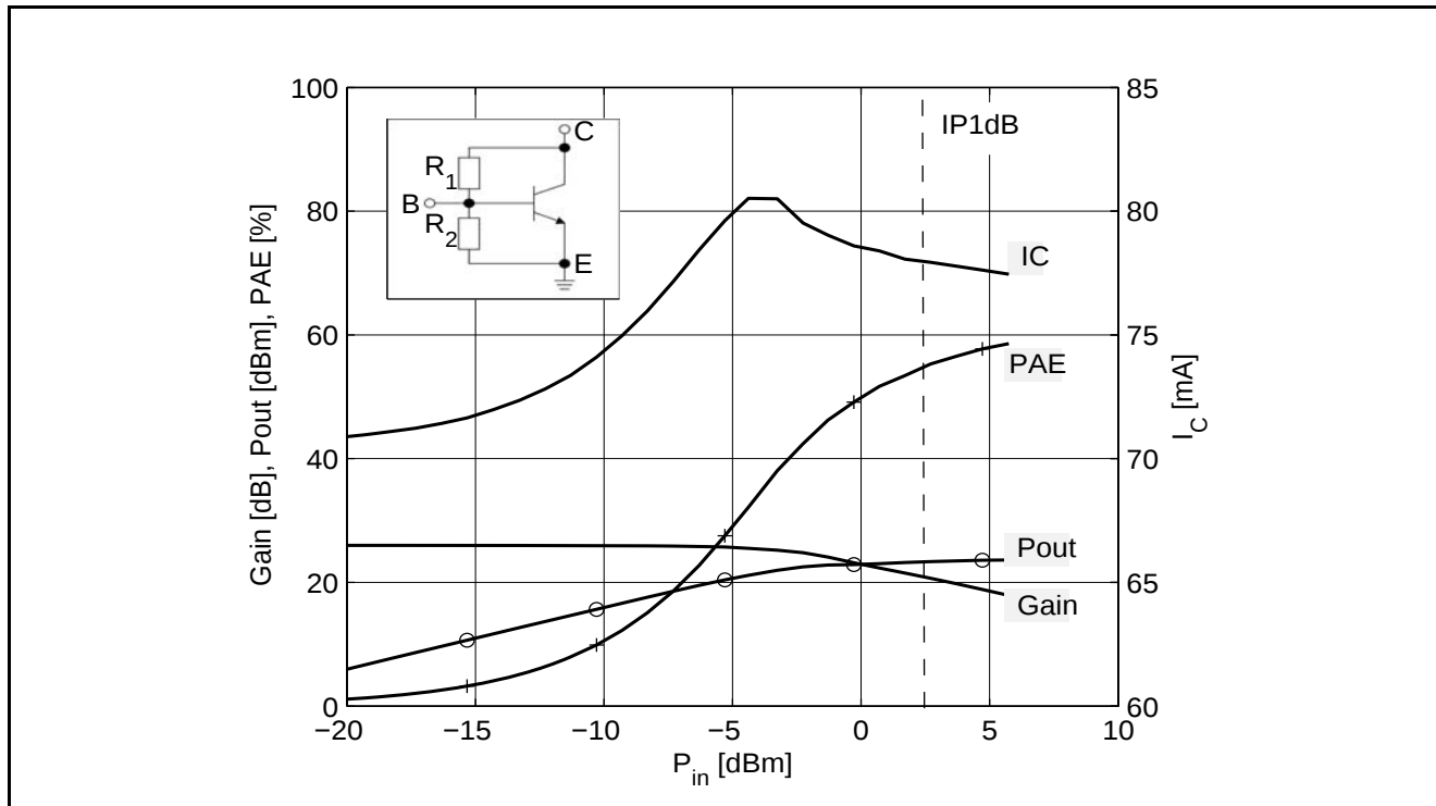
Figure 7-18 P_{out} , Gain, I_C , PAE vs. P_{in} at V_{CE} = 5 V, f = 0.9 GHz, Z_I = Z_{opt} , R_1 = 270 \Omega , R_2 = 8 k \Omega
