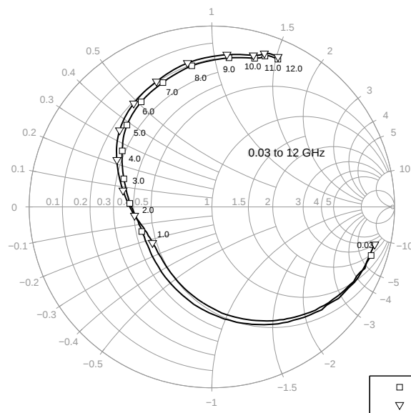
Figure 7-10 Output Reflection Coefficient S_{22} vs. f at V_{CE} = 5 V, I_C = Parameter
