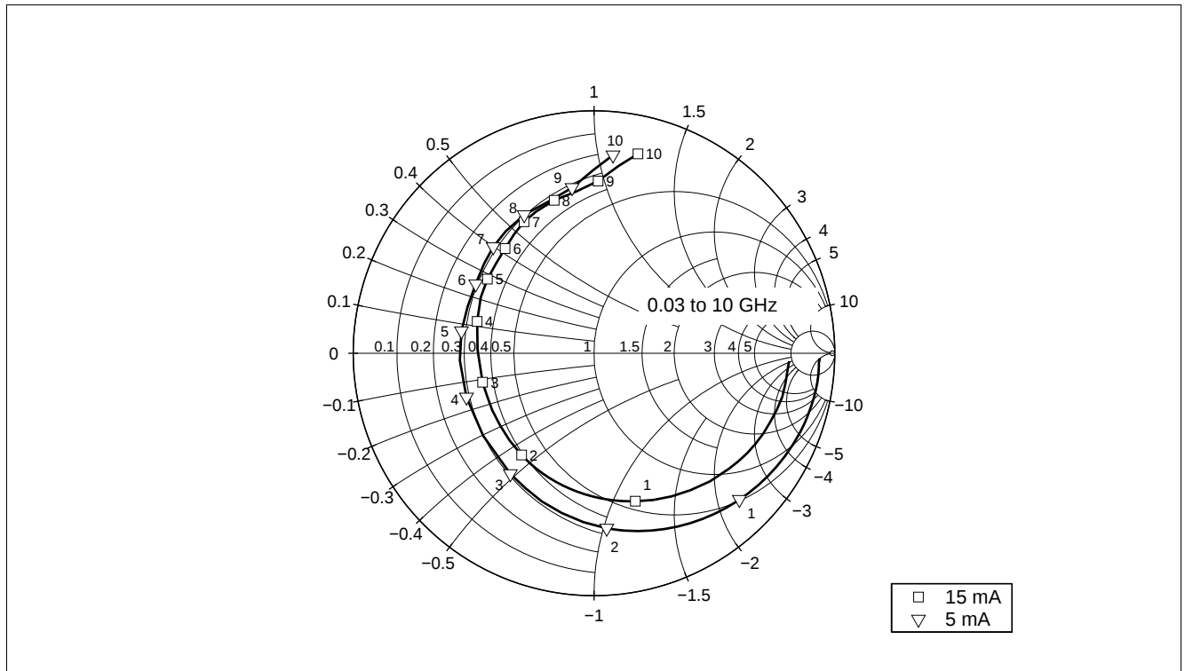
Figure 5-13 Input Matching S_{11} = f(f) , V_{CE} = 3 V, I_C = 5 / 15 mA
