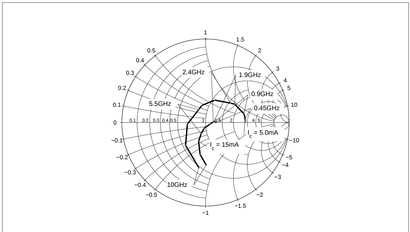
Figure 5-14 Source Impedance for Minimum Noise Figure Z_{opt} = f(f) , V_{CE} = 3 V, I_C = 5 / 15 mA
