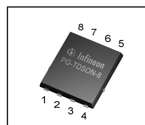
PG-TDSON-8-10
