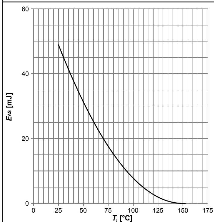
Diagram 11: Avalanche energy
