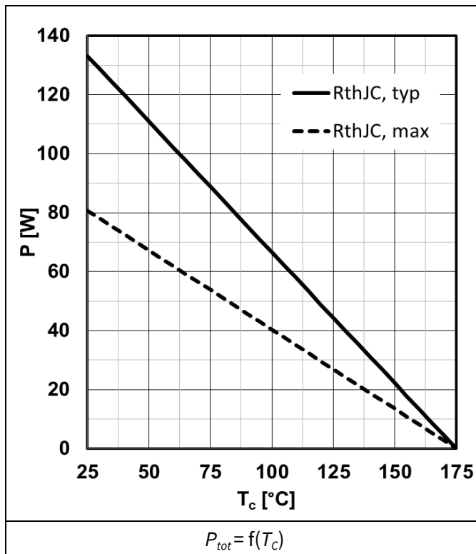
Figure 1 Power dissipation
