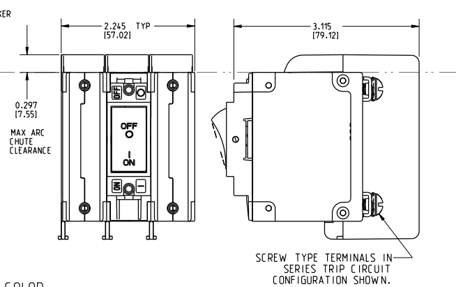
3-POLE (CF3,CG3,C13,C23) w/ ARC CHUTE BARRIER
