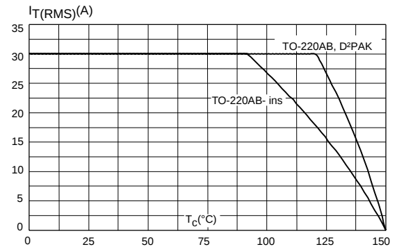
Figure 2: On-state RMS current versus case temperature
