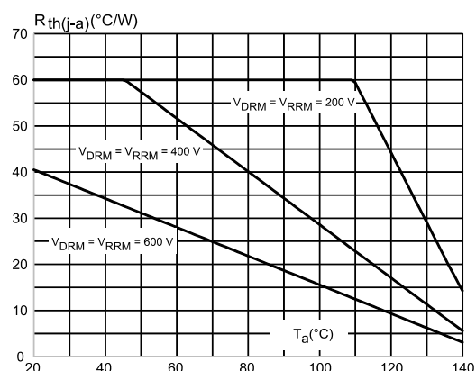
Figure 14: Acceptable junction to ambient thermal resistance versus repetitive peak off-state voltage and ambient temperature
