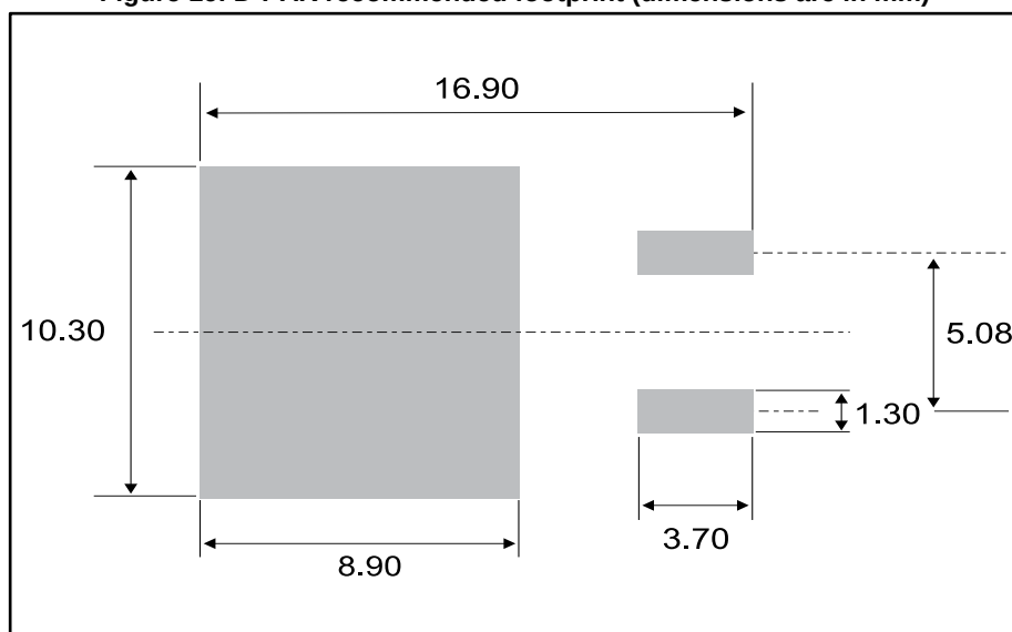
Figure 16: D 2 PAK recommended footprint (dimensions are in mm)
