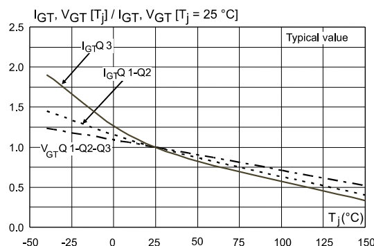
Figure 5: Relative variation of gate trigger current and gate trigger voltage versus junction temperature
