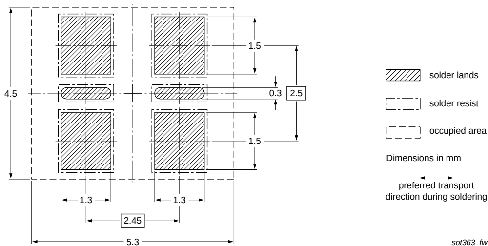
Fig 14. Wave soldering footprint PUMB1 (SOT363)
