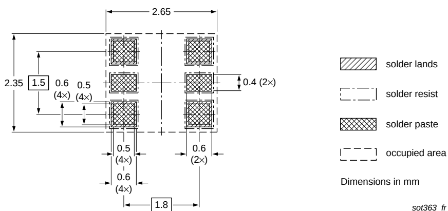
Fig 13. Reflow soldering footprint PUMB1 (SOT363)
