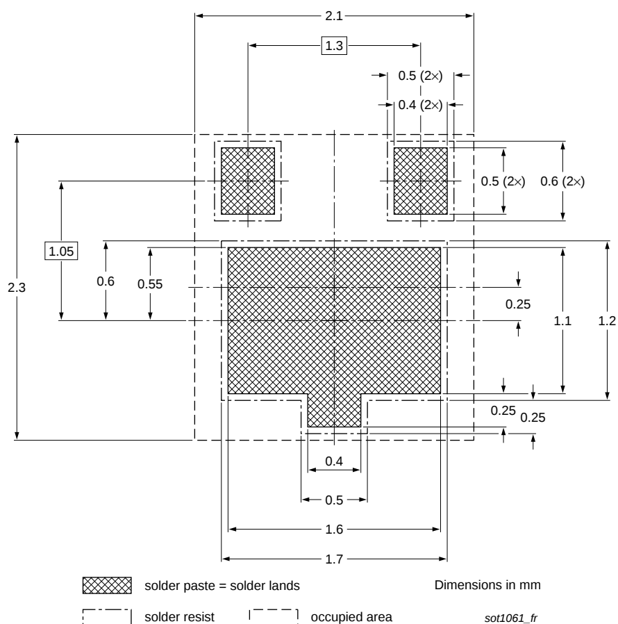
Fig 26. Reflow soldering footprint SOT1061 (HUSON3)
