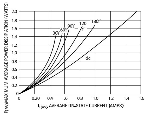
Figure 8. Power Dissipation
