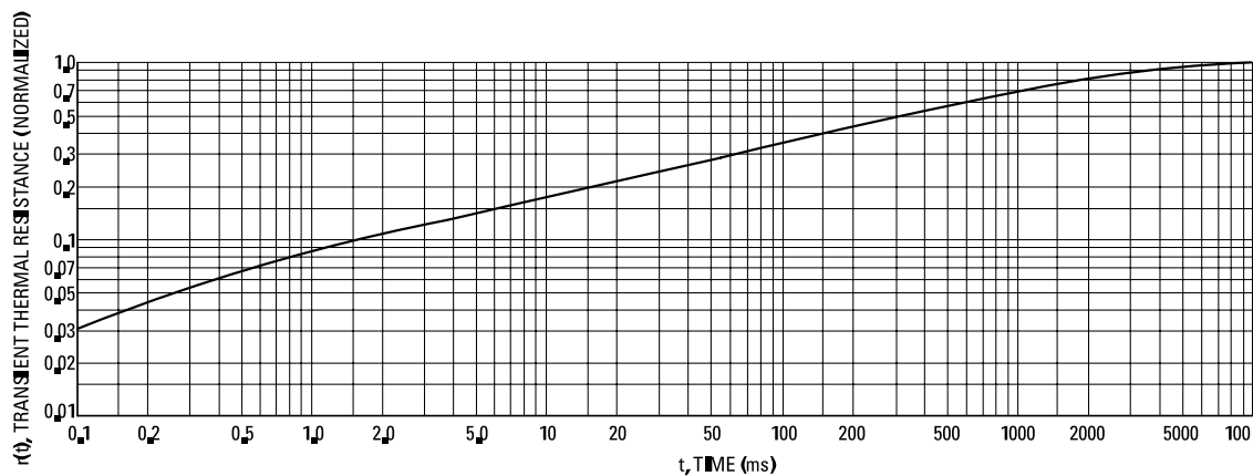
Figure 4. Thermal Response
