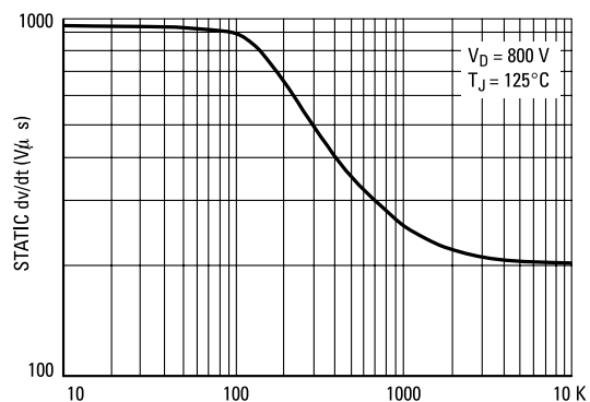
Figure 9. Exponential Static dv/dt vs Gate–Cathode Resistance
