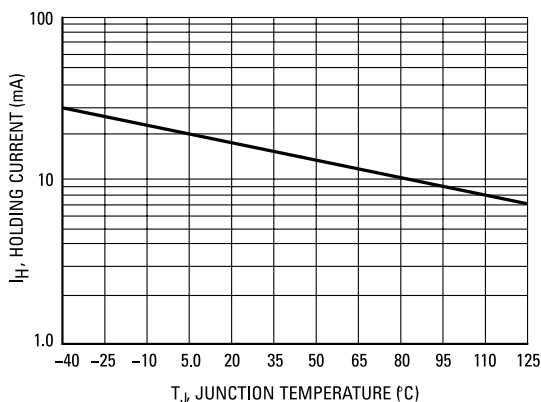
Figure 7. Typical Holding Current vs Junction Temperature
