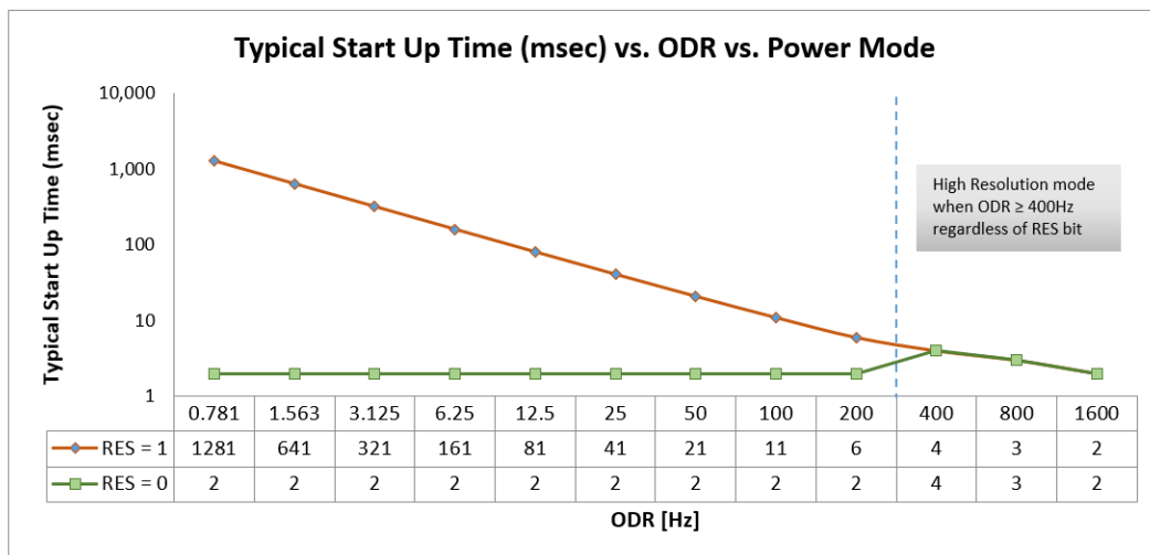
Figure 1: Typical Start Up Time
