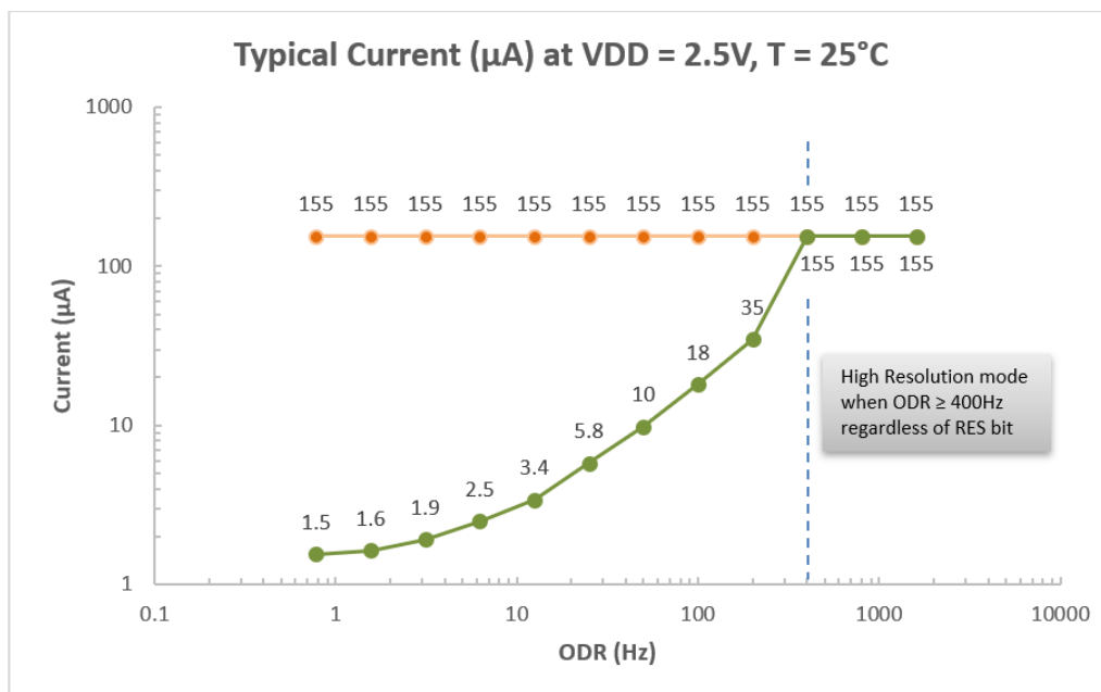
Figure 2: Current Profile
