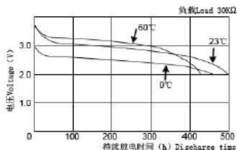
Discharge Characteristics on Temperature
