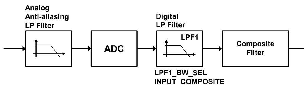
Figure 8. Accelerometer chain
