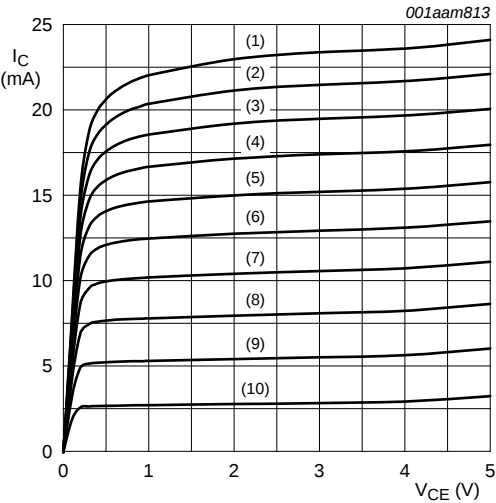
T_{amb} = 25\text{ }^{\circ}\text{C}. (1) I_B = 200\text{ }\mu\text{A} (2) I_B = 180\text{ }\mu\text{A} (3) I_B = 160\text{ }\mu\text{A} (4) I_B = 140\text{ }\mu\text{A} (5) I_B = 120\text{ }\mu\text{A} (6) I_B = 100\text{ }\mu\text{A} (7) I_B = 80\text{ }\mu\text{A} (8) I_B = 60\text{ }\mu\text{A} (9) I_B = 40\text{ }\mu\text{A} (10) I_B = 20\text{ }\mu\text{A}
