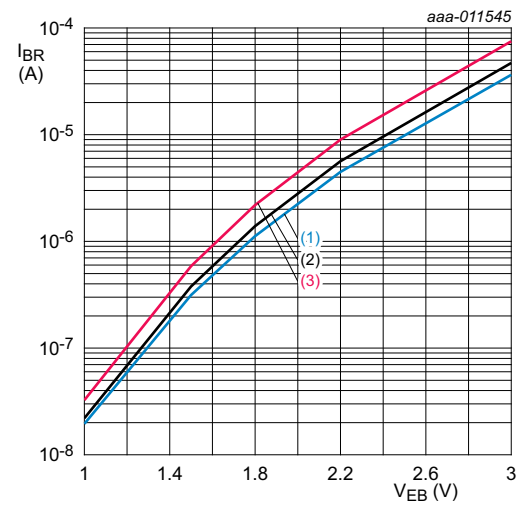
V_{CE} = 3 V. (1) T_{amb} = -40^\circ\text{C} (2) T_{amb} = +25^\circ\text{C} (3) T_{amb} = +125^\circ\text{C}
