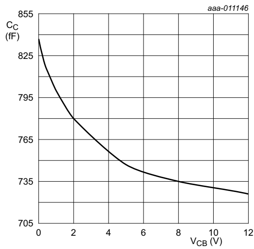
I_C = 0 mA; f = 1 MHz; T_{amb} = 25^\circ\text{C} .
