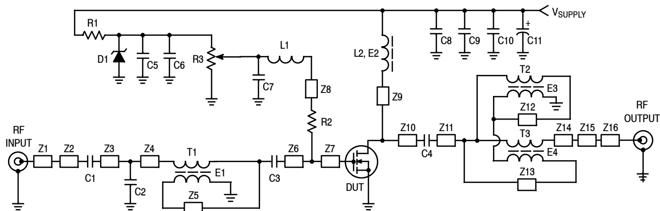
Figure 25. MRFE6VS25L Broadband Reference Circuit Schematic — 30-512 MHz
