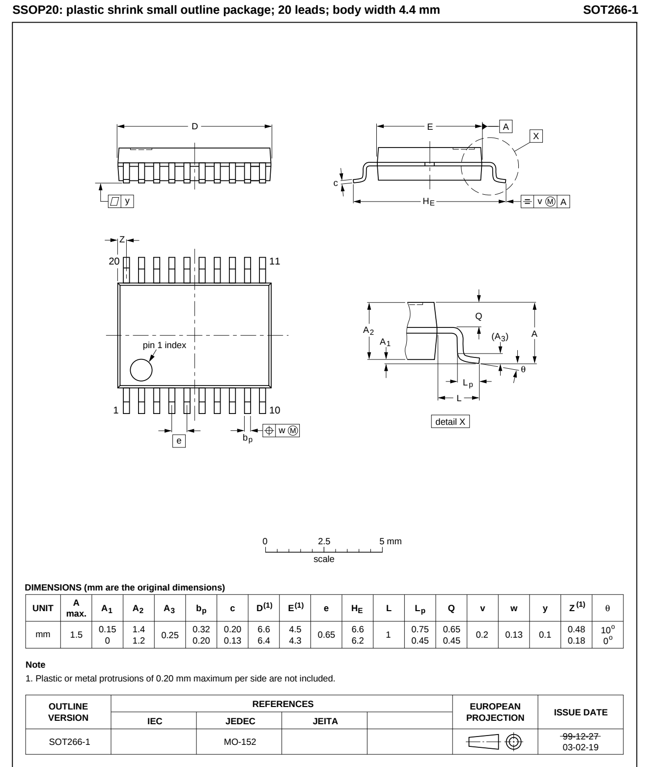
Fig 19. Package outline SOT266-1 (SSOP20)
