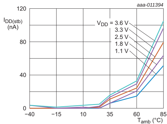
Fig 16. Standby supply current versus ambient temperature
