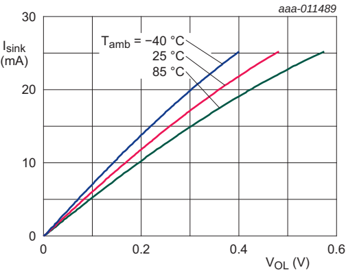
c. V DD = 2.5 V
