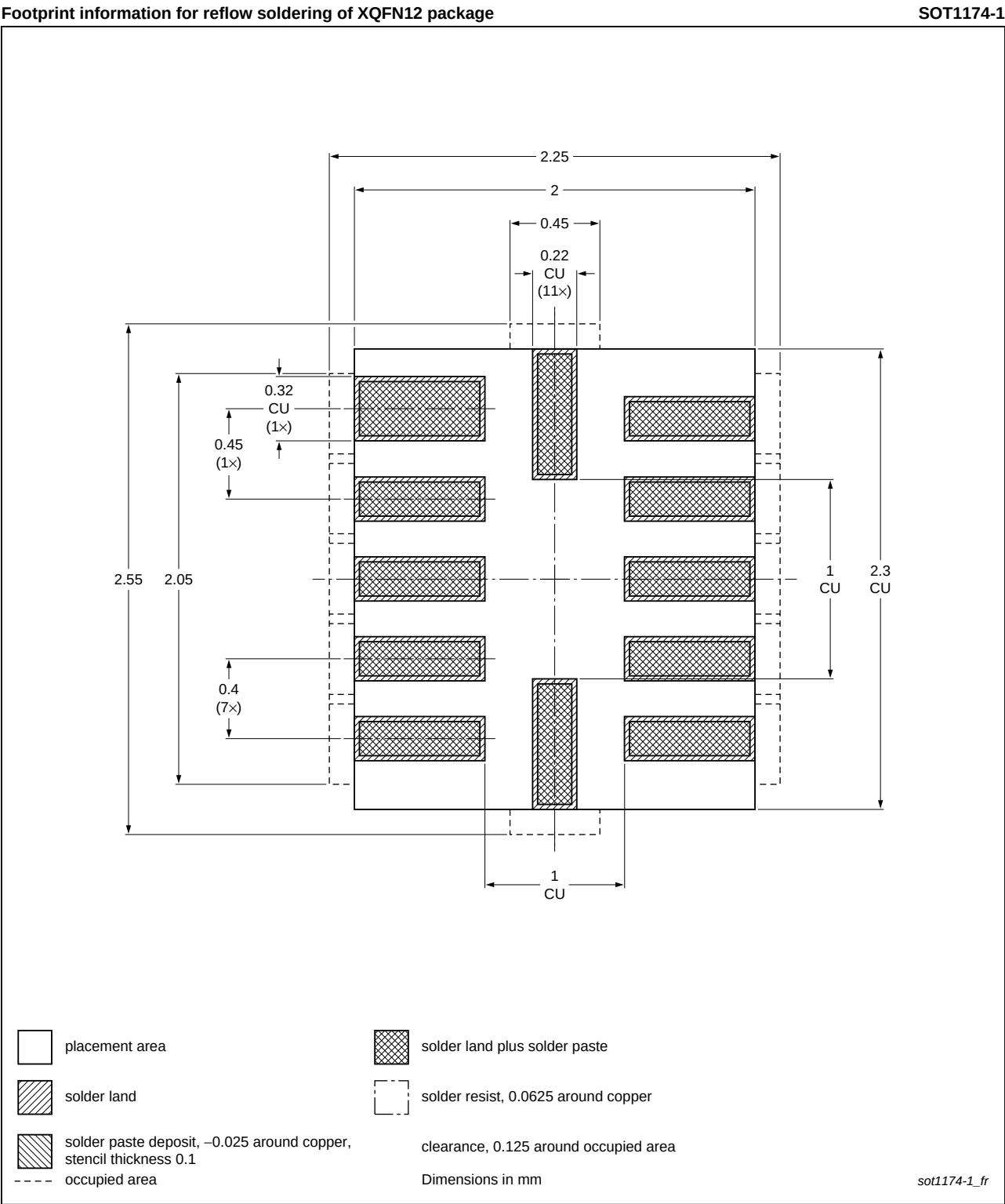
Fig 30. PCB footprint for SOT1174-1 (XQFN12); reflow soldering
