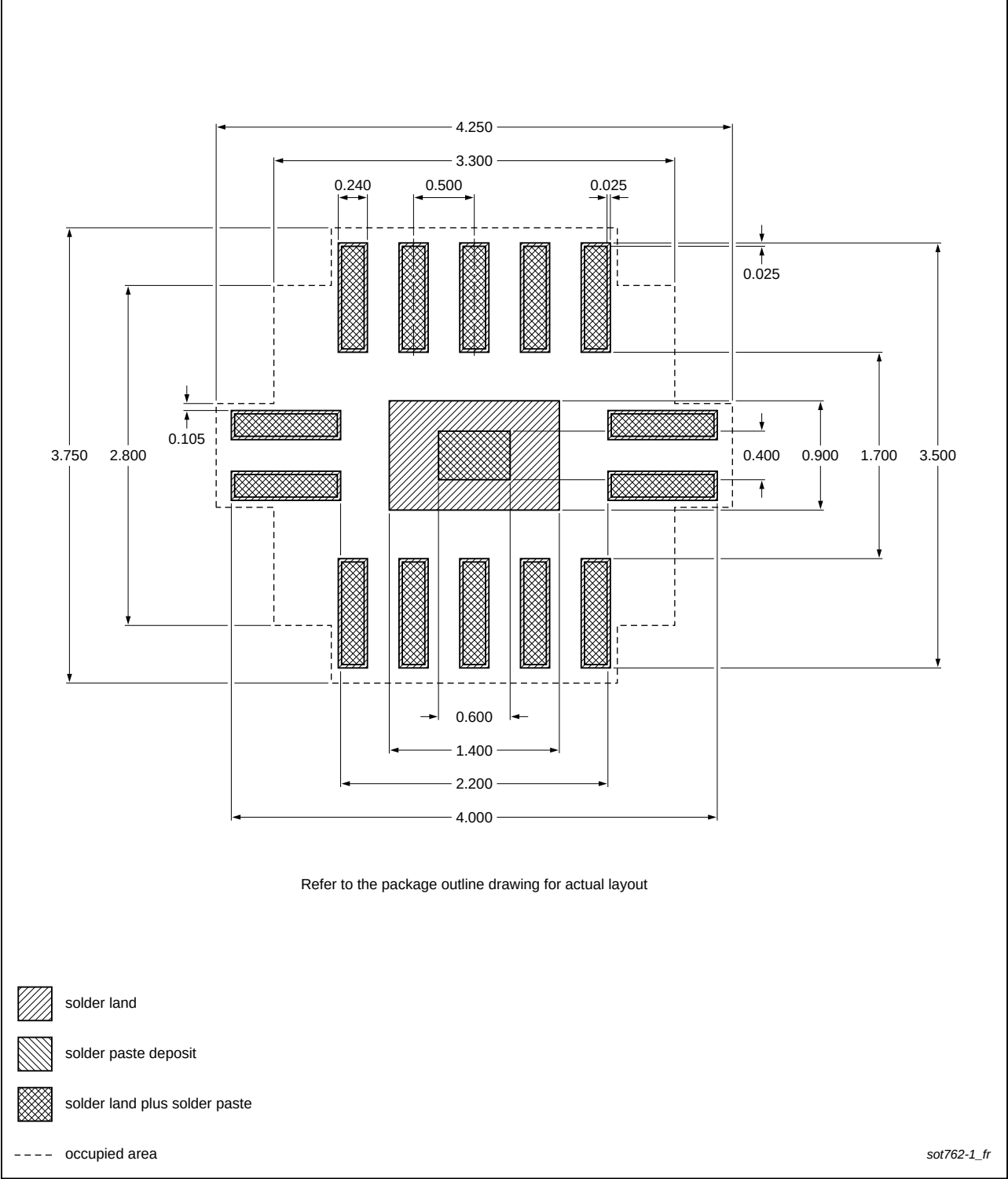
Fig 31. PCB footprint for SOT762-1 (DHVQFN14); reflow soldering
