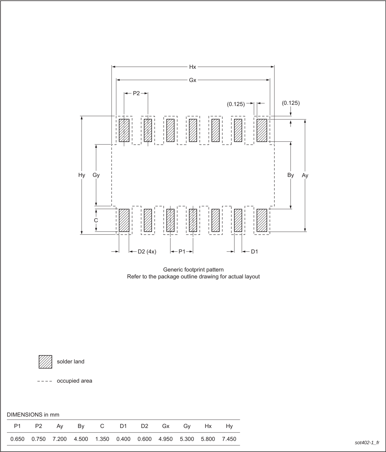
Fig 32. PCB footprint for SOT402-1 (TSSOP14); reflow soldering
