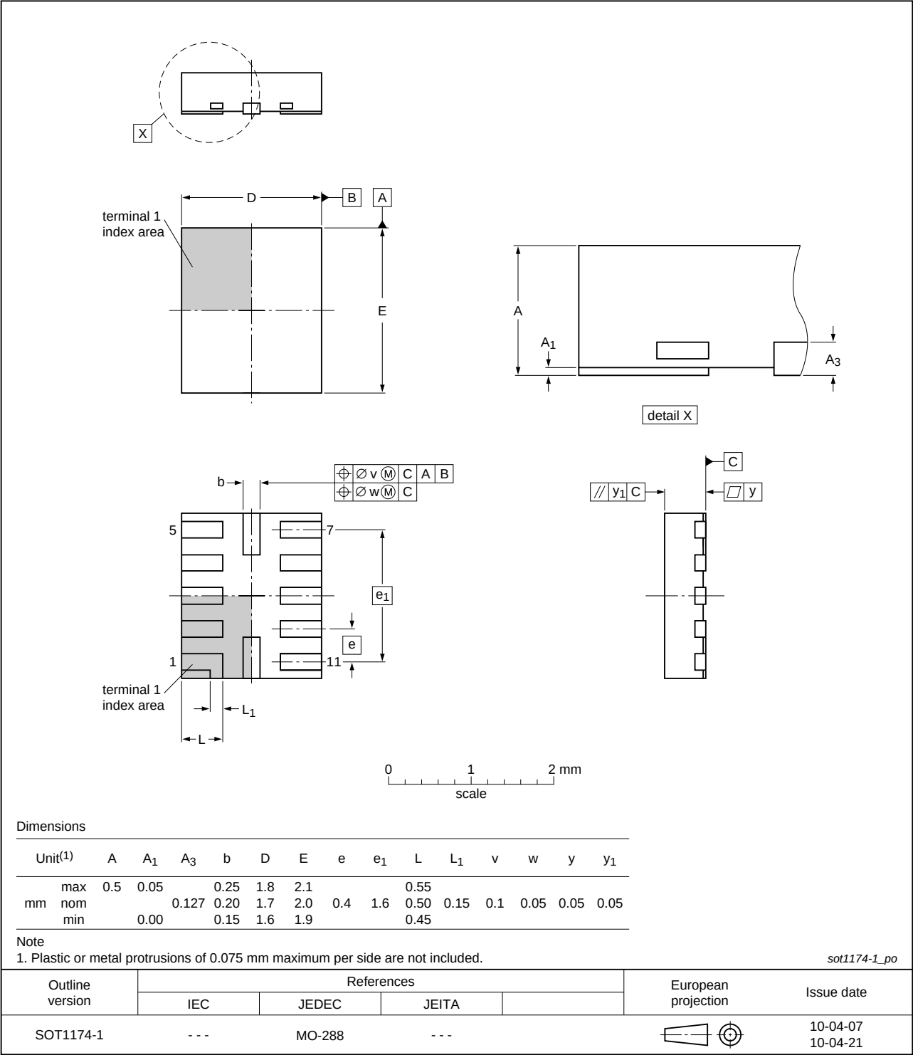
Fig 26. Package outline SOT1174-1 (XQFN12)
