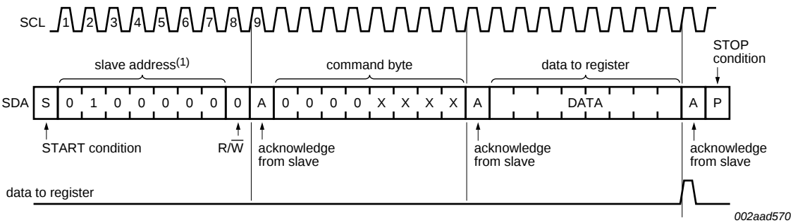
Fig 14. Write to Polarity inversion, Bus-hold enable, Pull-up/pull-down select, Configuration, Interrupt mask and Interrupt status registers
