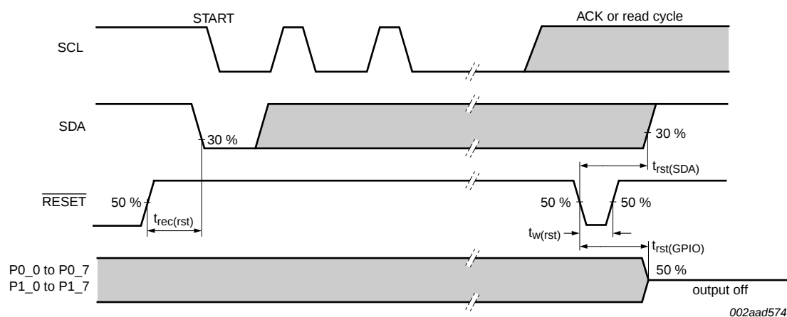
Fig 23. Reset timing
