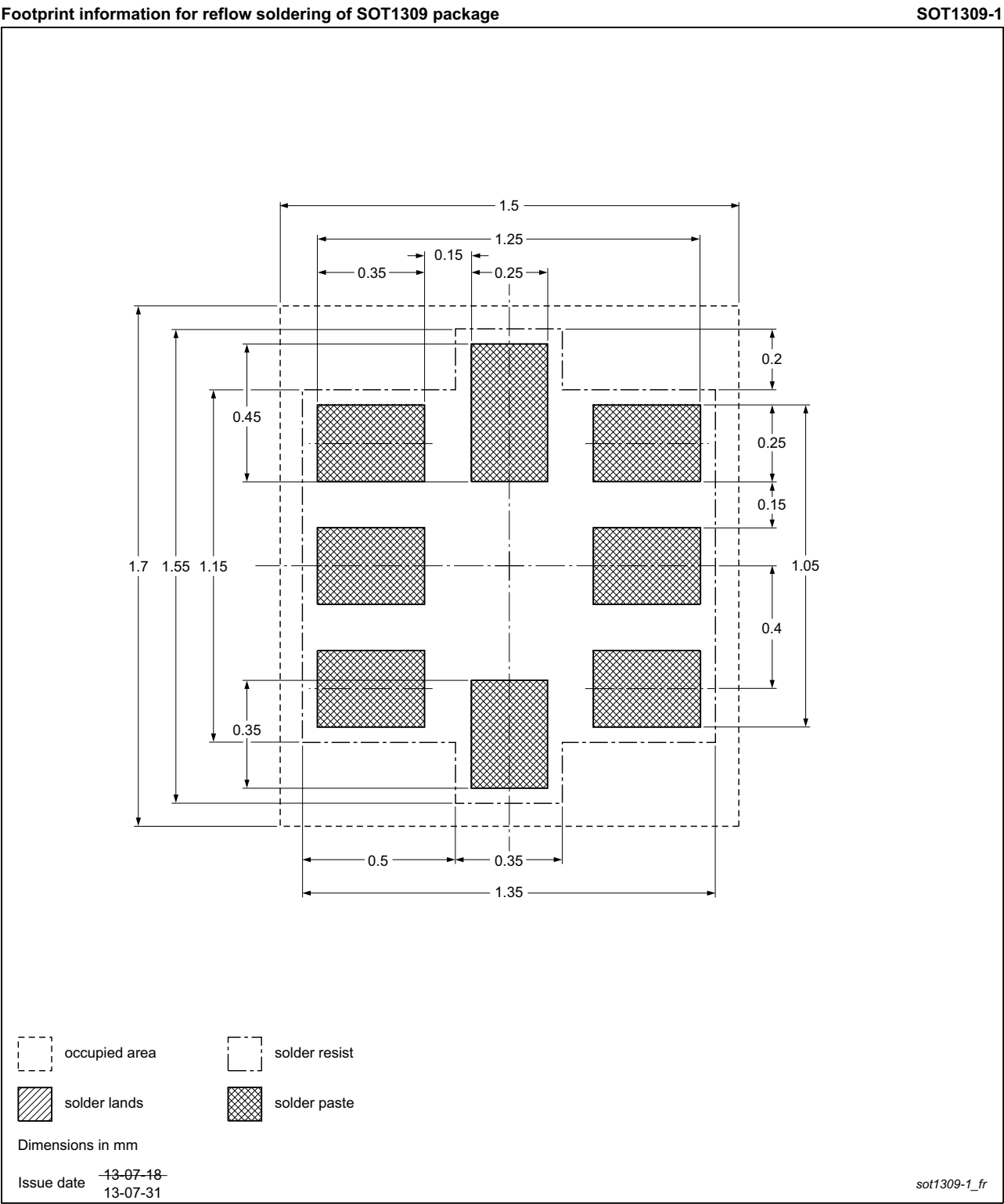
Fig 31. PCB footprint for SOT1309-1 (XQFN8); reflow soldering
