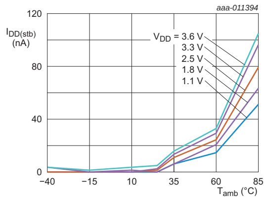
Fig 16. Standby supply current versus ambient temperature
