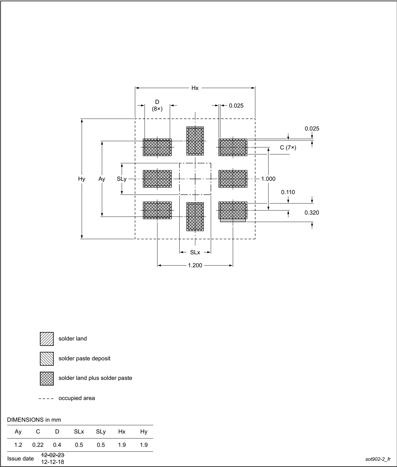
Footprint information for reflow soldering of XQFN8 package
