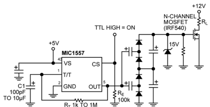
Figure 8. Charge Pump
