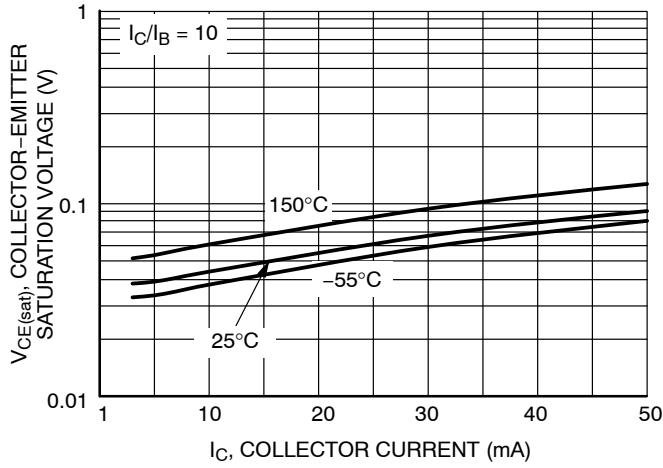
Figure 72. V_{CE(sat)} vs. I_C
