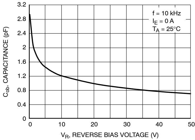
Figure 69. Output Capacitance
