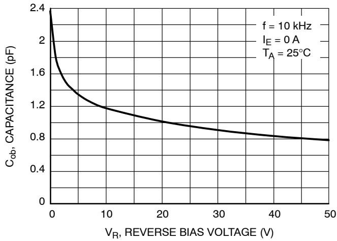
Figure 74. Output Capacitance
