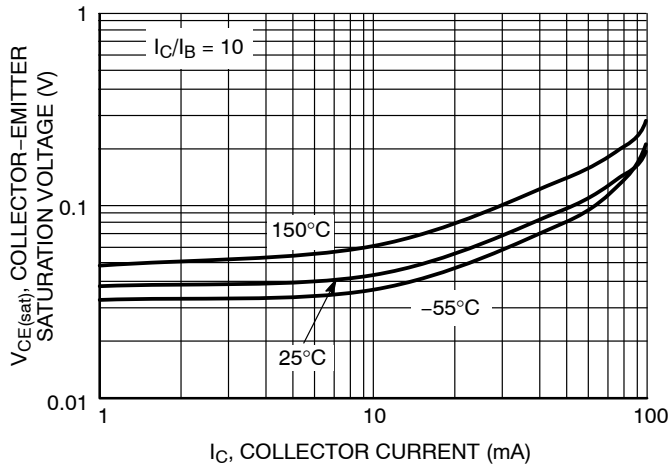
Figure 67. V_{CE(sat)} vs. I_C
