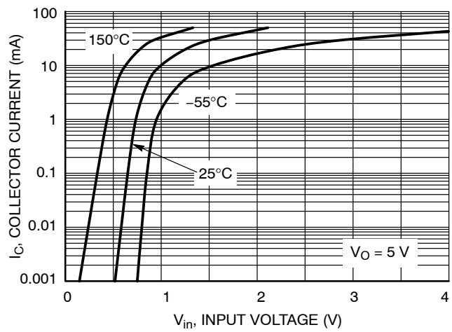
Figure 70. Output Current vs. Input Voltage
