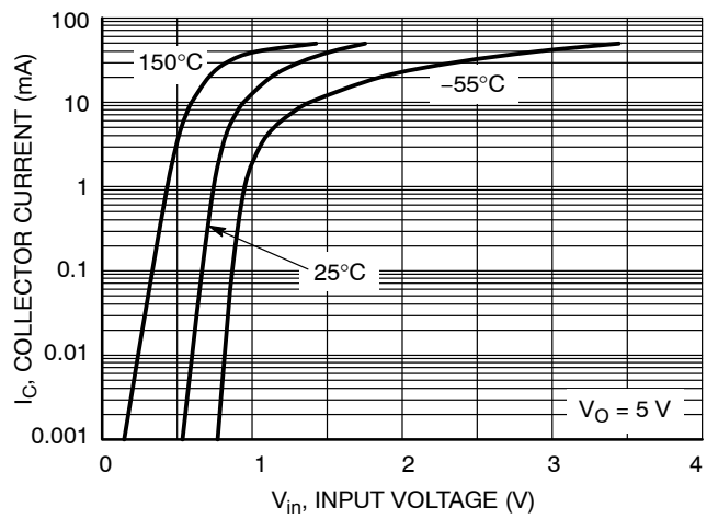
Figure 75. Output Current vs. Input Voltage
