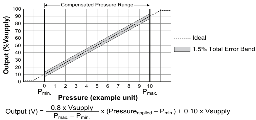
Figure 3. Transfer Function Limits 1
