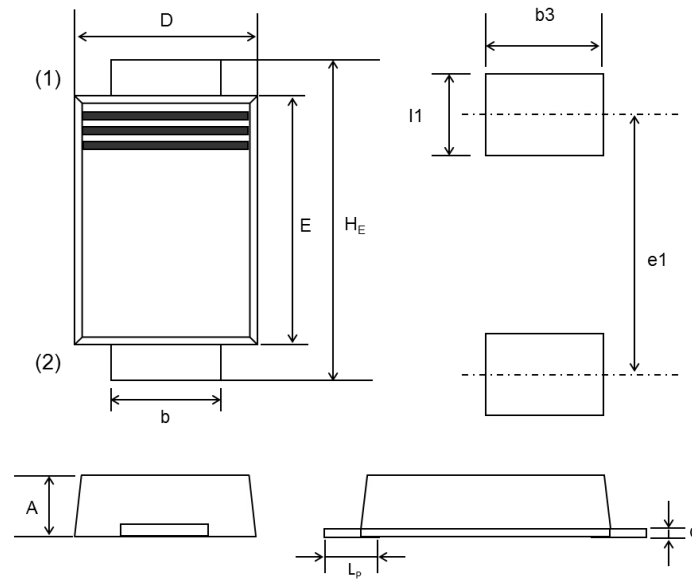
SOD-128, (PMD™)
