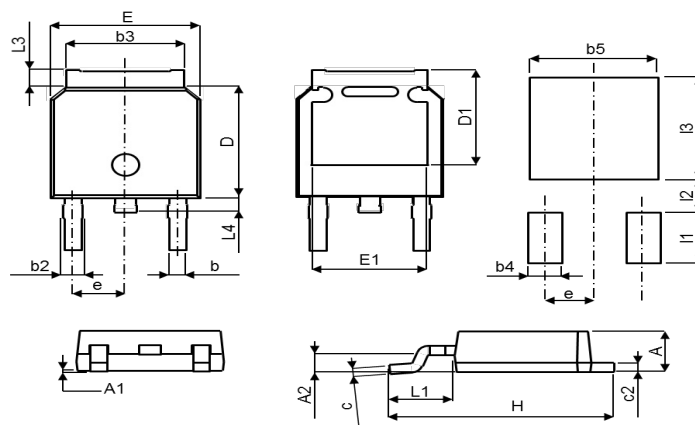
TO-252, (TO-252)
