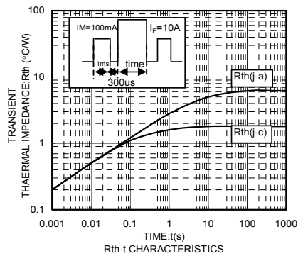
R_{\theta} - t CHARACTERISTICS
