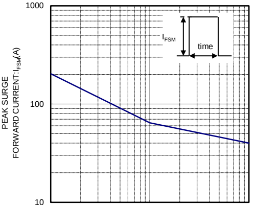
I_{FSM} - t CHARACTERISTICS
