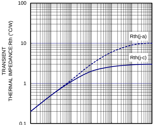
R_{th} - t CHARACTERISTICS
