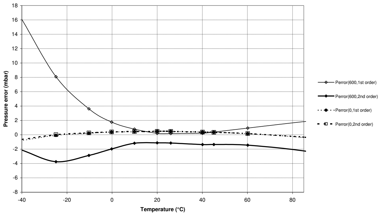
Pressure Error Accuracy vs temperature (typical) for MS5536-CPJU
