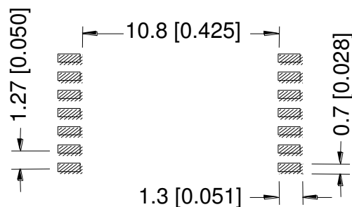
Fig. 9: Recommended pad-layout for MS5536-CPJU / MS5536-CNJU
