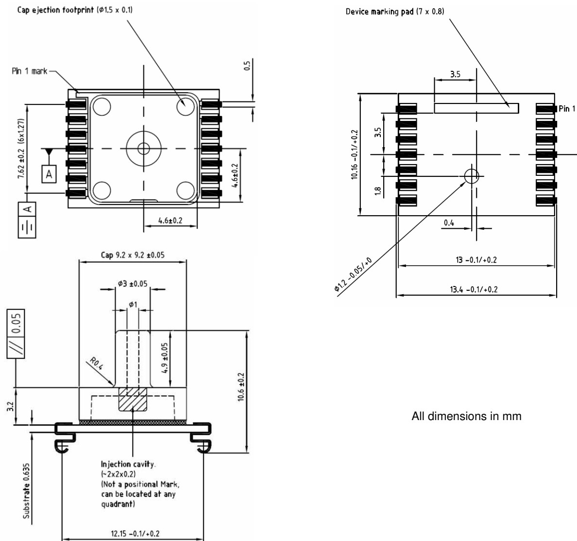
Fig. 8: Device package outlines of MS5536-CPJU / MS5536-CNJU
