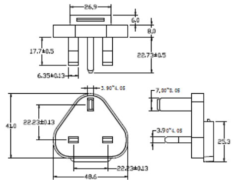
UK PIN
