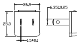
US PIN
